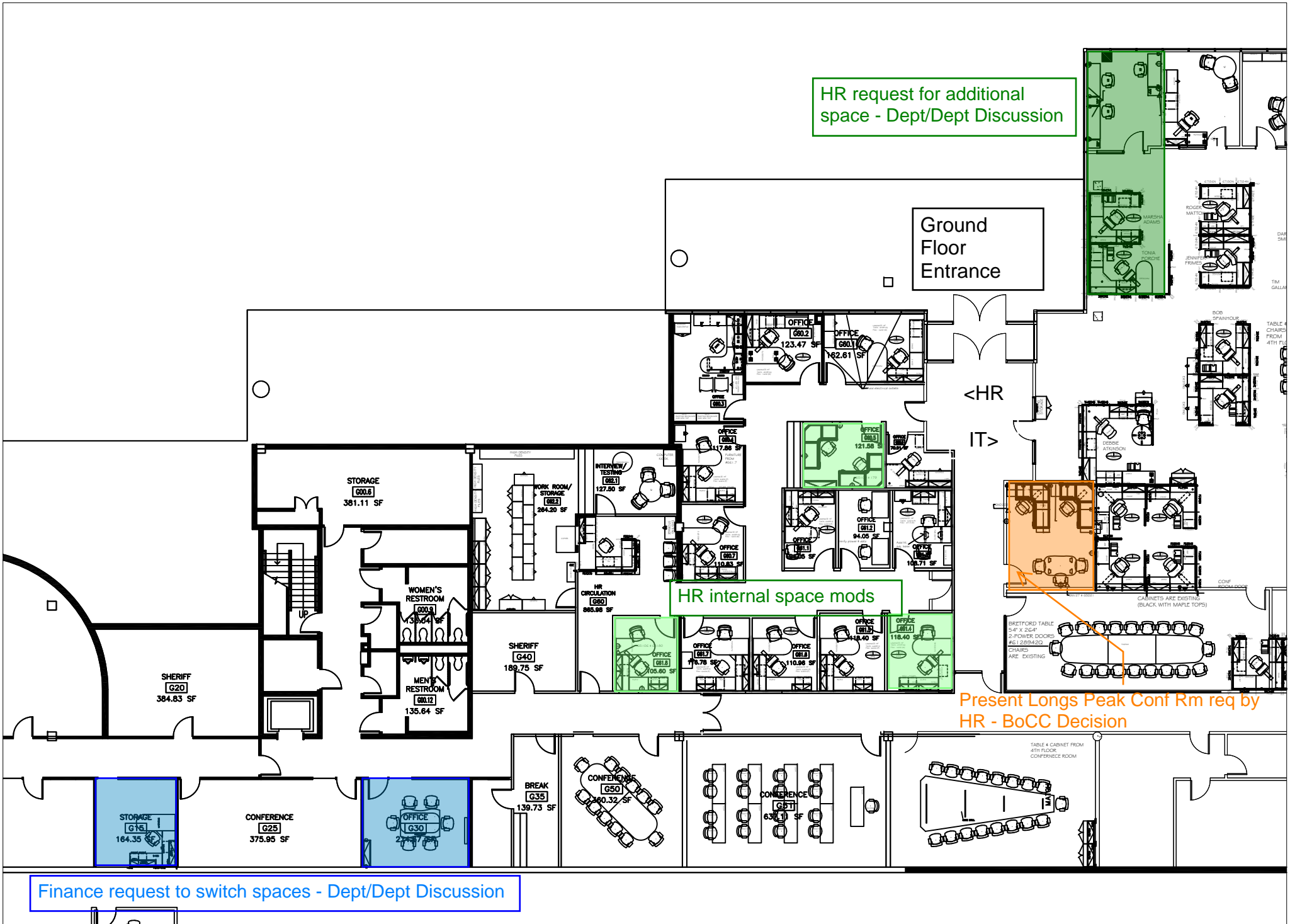
Admin Ground Floor Proposed Modifications 2026
